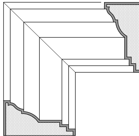
CASING DETAIL
