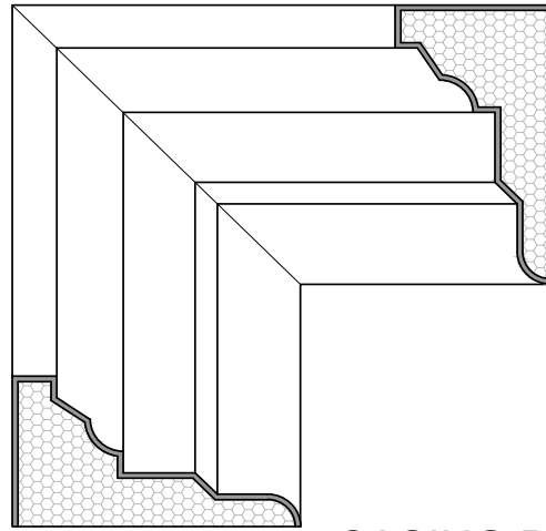
CASING DETAIL
