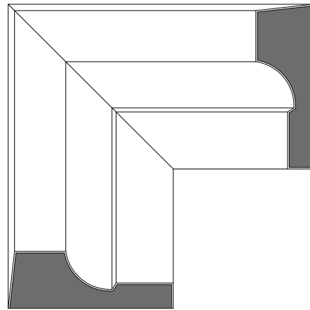
CASING DETAIL
