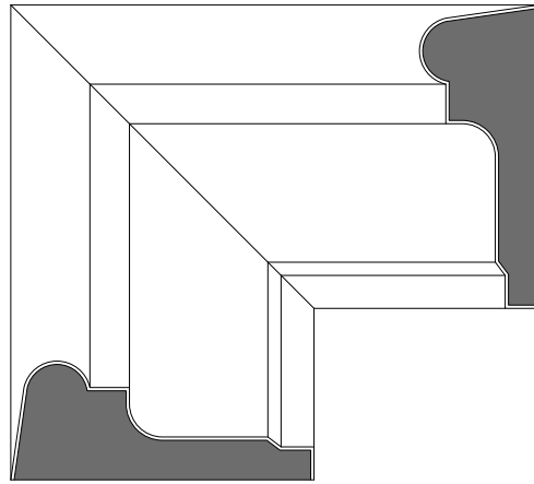
CASING DETAIL
