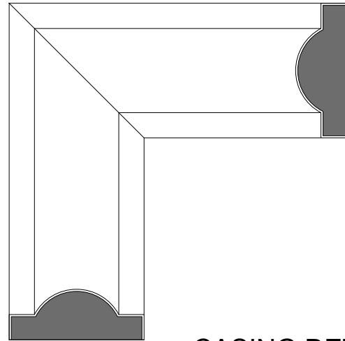
CASING DETAIL
