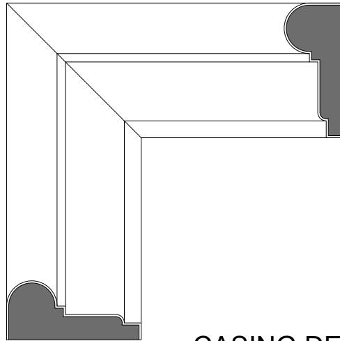
CASING DETAIL
