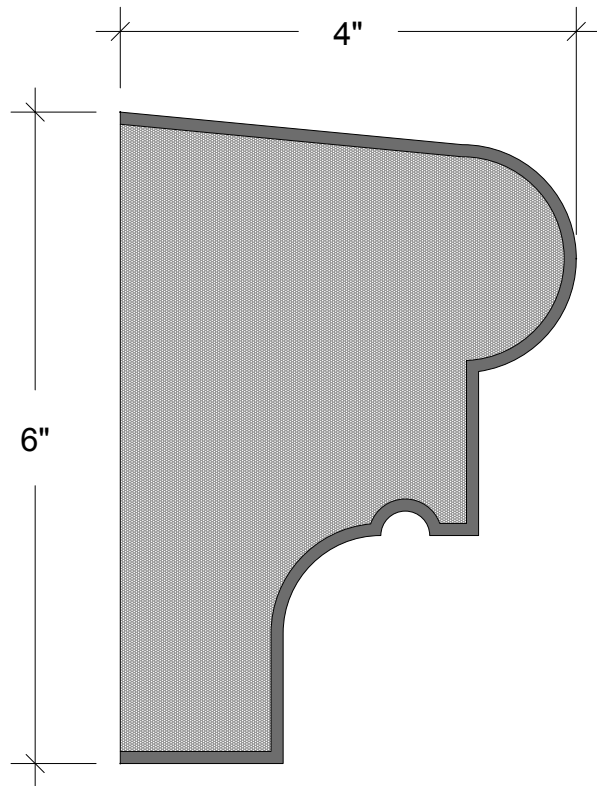
SECTION
