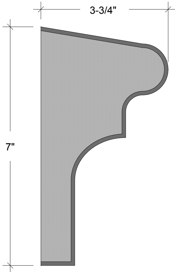
SECTION
