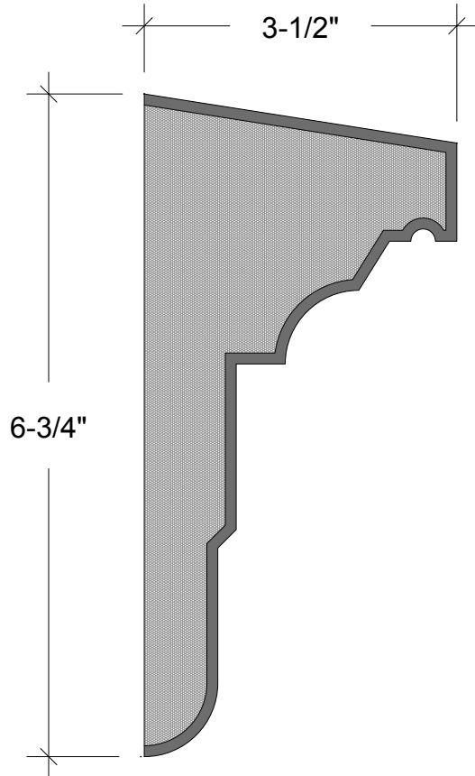
SECTION
