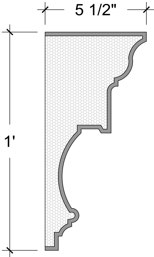
SECTION
