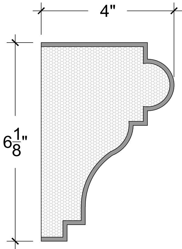
SECTION
