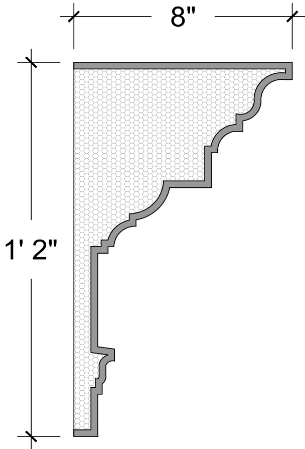
SECTION
